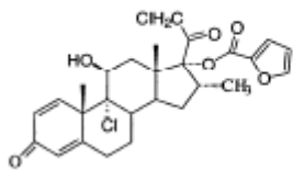
FIGURE 1.1: MOMETASONE FUROATE (SCH 32088)
